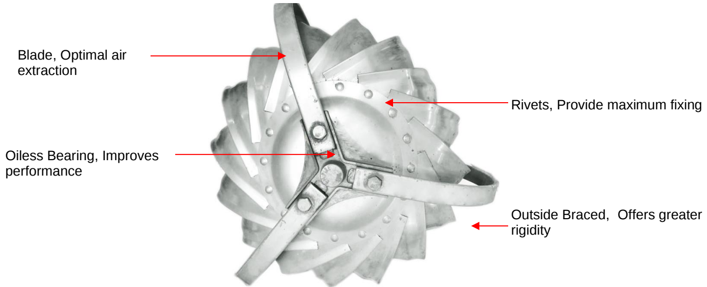
EmpiStainless, Top view
