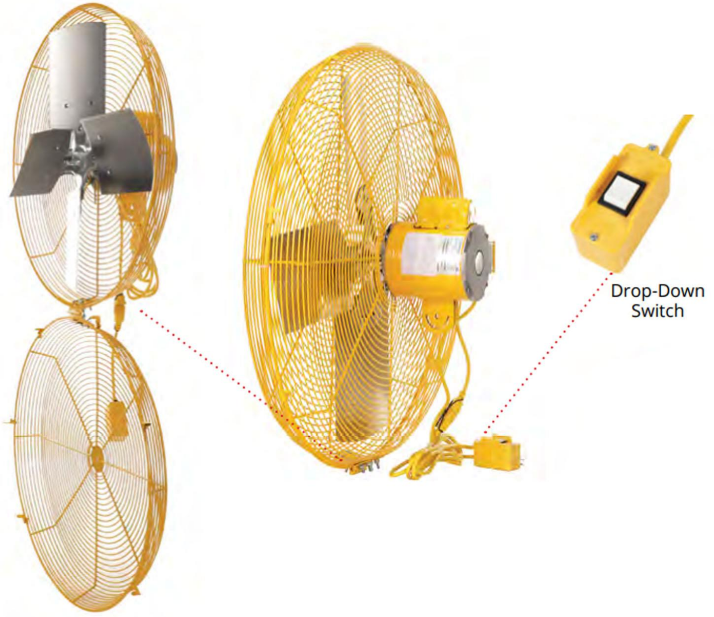
Hinged Guard
