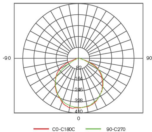
cd/1000lm Curva
