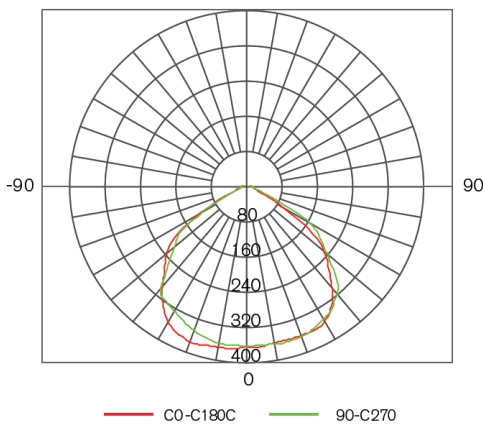
cd/1000 lm Curva
