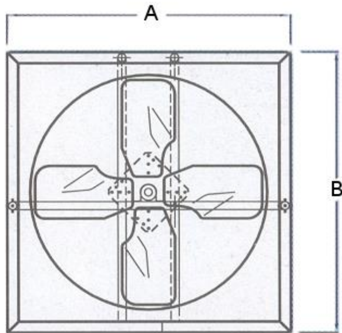
VISTA FRONTAL
